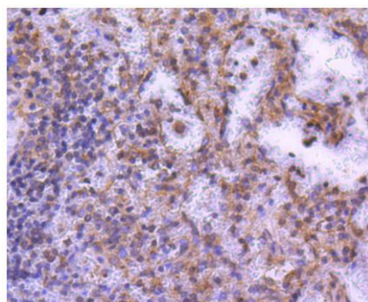
Fig. 3. Immunohistochemical analysis of paraffin-embedded human spleen tissue using anti-MEK2 antibody. Counter stained with hematoxylin.
