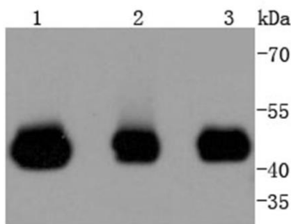
Fig. 1. Western blot analysis of MEK2 on different lysates using anti-MEK2 antibody at 1/1,000 dilution. Positive control: Lane 1: Jurkat; Lane 2: HeLa; Lane 3: 293T
