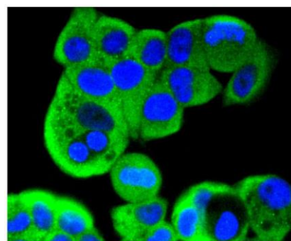
Fig. 2. ICC staining MEK2 in MCF-7 cells (green). The nuclear counter stain is DAPI (blue). Cells were fixed in paraformaldehyde, permeabilised with 0.25% Triton X-100/PBS.
