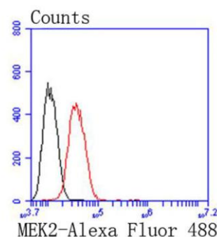
Fig. 4. Flow cytometric analysis of HeLa cells with MEK2 antibody at 1/50 dilution (red) compared with an unlabelled control (cells without incubation with primary antibody; black). Alexa Fluor 488-conjugated goat anti rabbit IgG was used as the secondary antibody.
